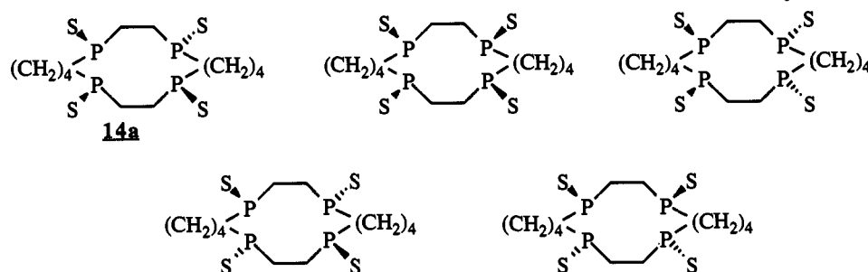
Scheme 1. Possible Isomers of 14
