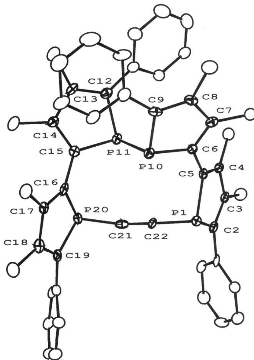
Figure 1. ORTEP drawing of one molecule of 6 . Vibrational ellipsoids are scaled to enclose 50% of the electronic density. Hydrogen atoms are omitted for clarity. Principal bond distances ( \text{\AA} ) and angles (deg): P 1 –C 2 1.820(7), P 1 –C 5 1.830(9), P 1 –C 22 1.753(7), C 5 –C 6 1.46(1), C 6 –P 10 1.795(8), P 10 –C 9 1.799(7), P 10 –P 11 2.204(3), P 11 –C 12 1.799(9), P 11 –C 15 1.789(7), C 15 –C 16 1.48(1), C 16 –P 20 1.836(7), P 10 –C 19 1.819(8), P 20 –C 21 1.789(9), C 21 –C 22 1.21(1); C 2 –P 1 –C 5 91.5(4), C 5 –P 1 –C 22 101.1(4), P 1 –C 5 –C 6 120.7(6), C 5 –C 6 –P 10 121.2(5), C 6 –P 10 –C 5 92.2(3), C 6 –P 10 –P 11 100.5(3), P 10 –P 11 –C 15 101.1(3), C 12 –P 11 –C 15 91.0(4), P 11 –C 15 –C 16 121.3(6), C 15 –C 16 –P 20 121.0(5), C 16 –P 20 –C 15 90.5(4), C 16 –P 20 –C 21 100.1(3), P 20 –C 21 –C 22 170.2(8), P 1 –C 21 –C 22 173.5(6).
